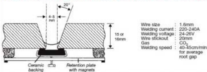
B Downhand position, root pass with FILARC basic flux-cored wire PZ6130HS, 1.6mm in CO 2 gas
