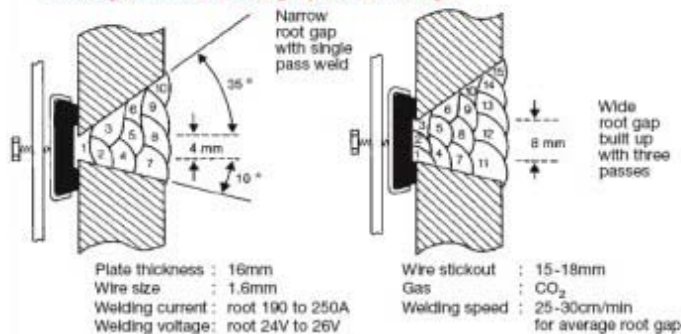
C Horizontal-vertical position, all passes with FILARC basic flux-cored wire PZ6130HS, 1.6mm in CO 2 gas or mixed gas. Decrease arc voltage by 1-2V for mixed gas.
